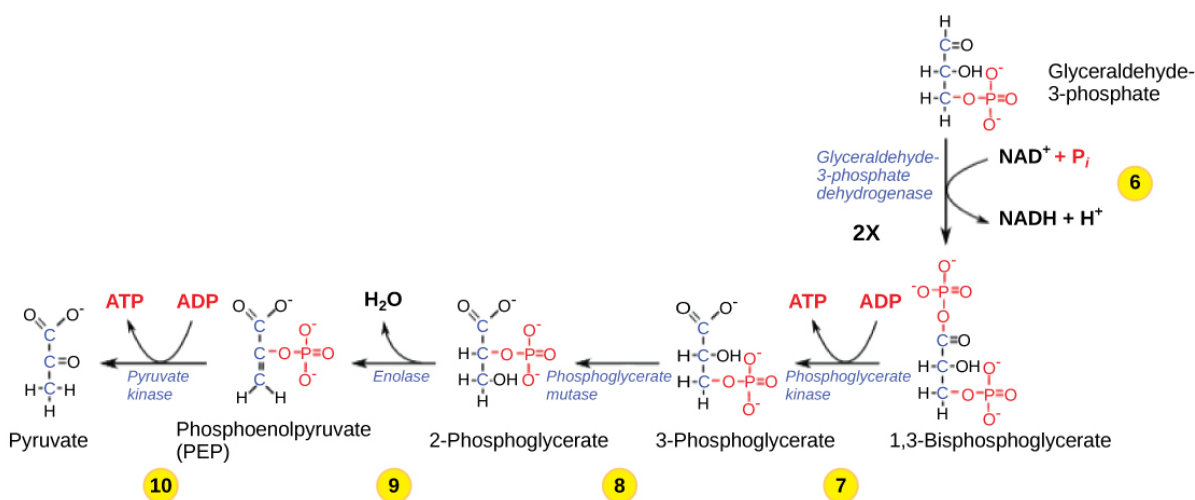
Figure 7.7 The second half of glycolysis involves phosphorylation without ATP investment (step 6) and produces two NADH and four ATP molecules per glucose.
